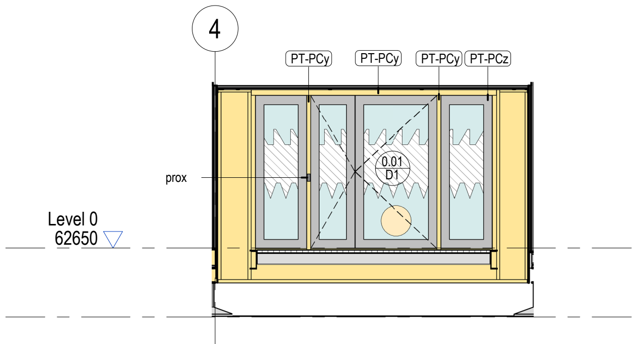
4 East Entry Link West Elevation 1 : 50
