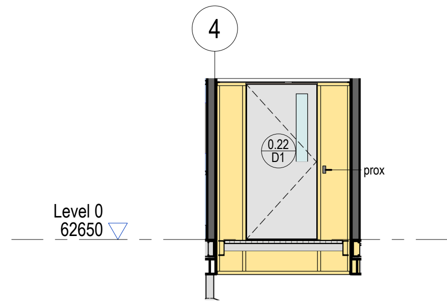
7 West Entry Link East Elevation 1 : 50
