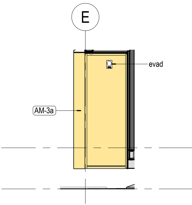
6 East Entry Link South Elevation 1 : 50
