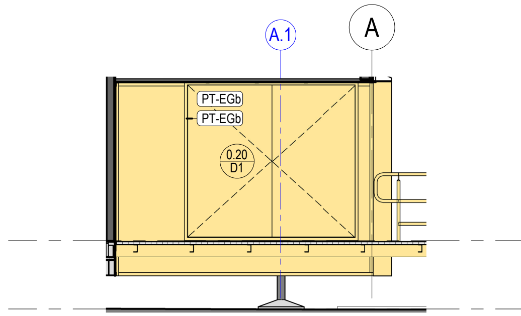
9 West Entry Link South Elevation 1 : 50
