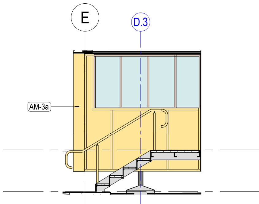
3 Stair South Elevation 1 : 50
