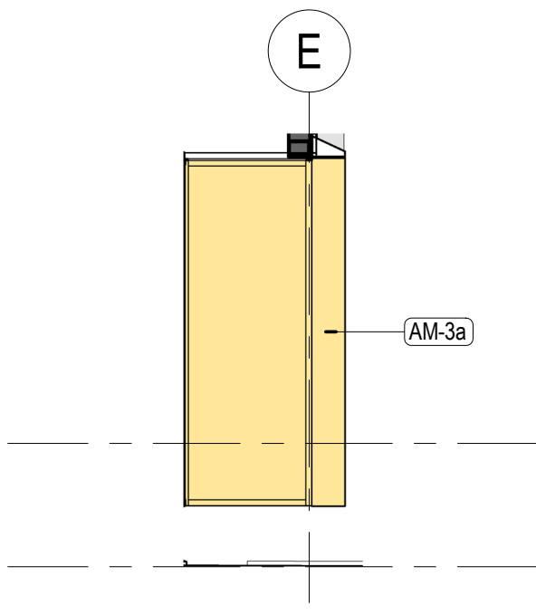
5 East Entry Link North Elevation 1 : 50
