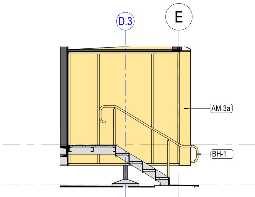
2 Stair 1 North Elevation 1 : 50
